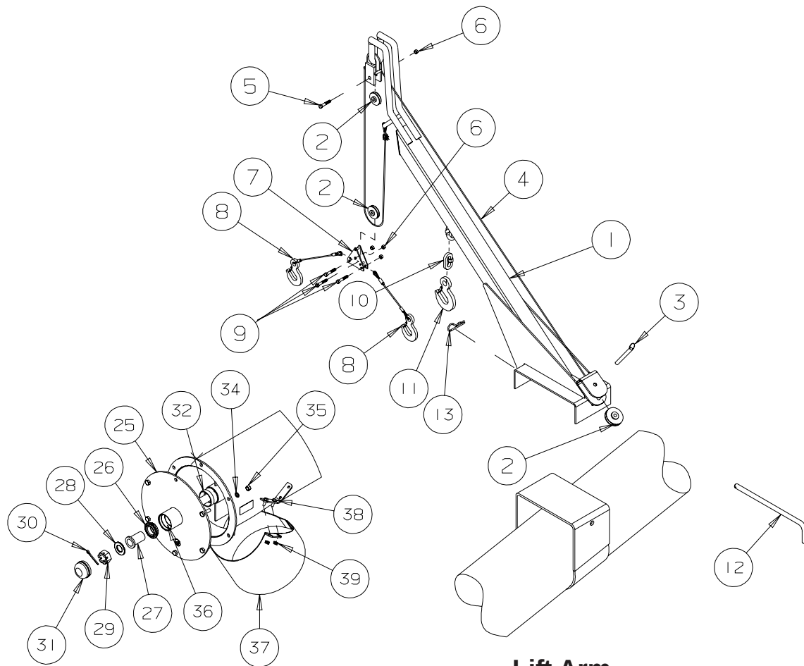
Upper Tube Head End Assembly
